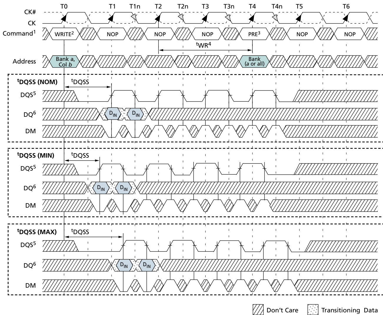
Figure 42: WRITE-to-PRECHARGE – Interrupting
