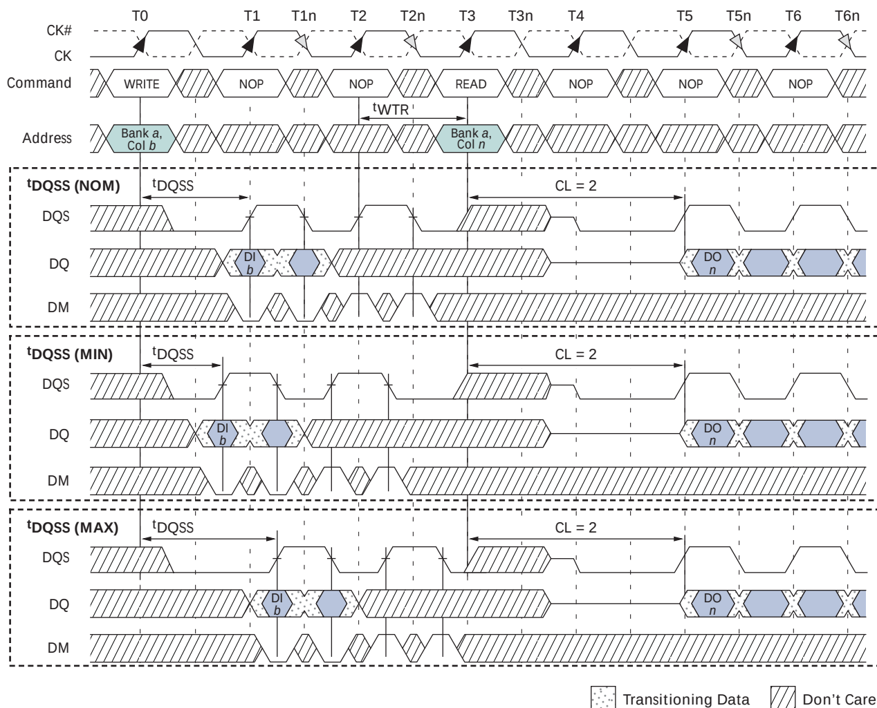
Figure 44: WRITE-to-READ – Interrupting
