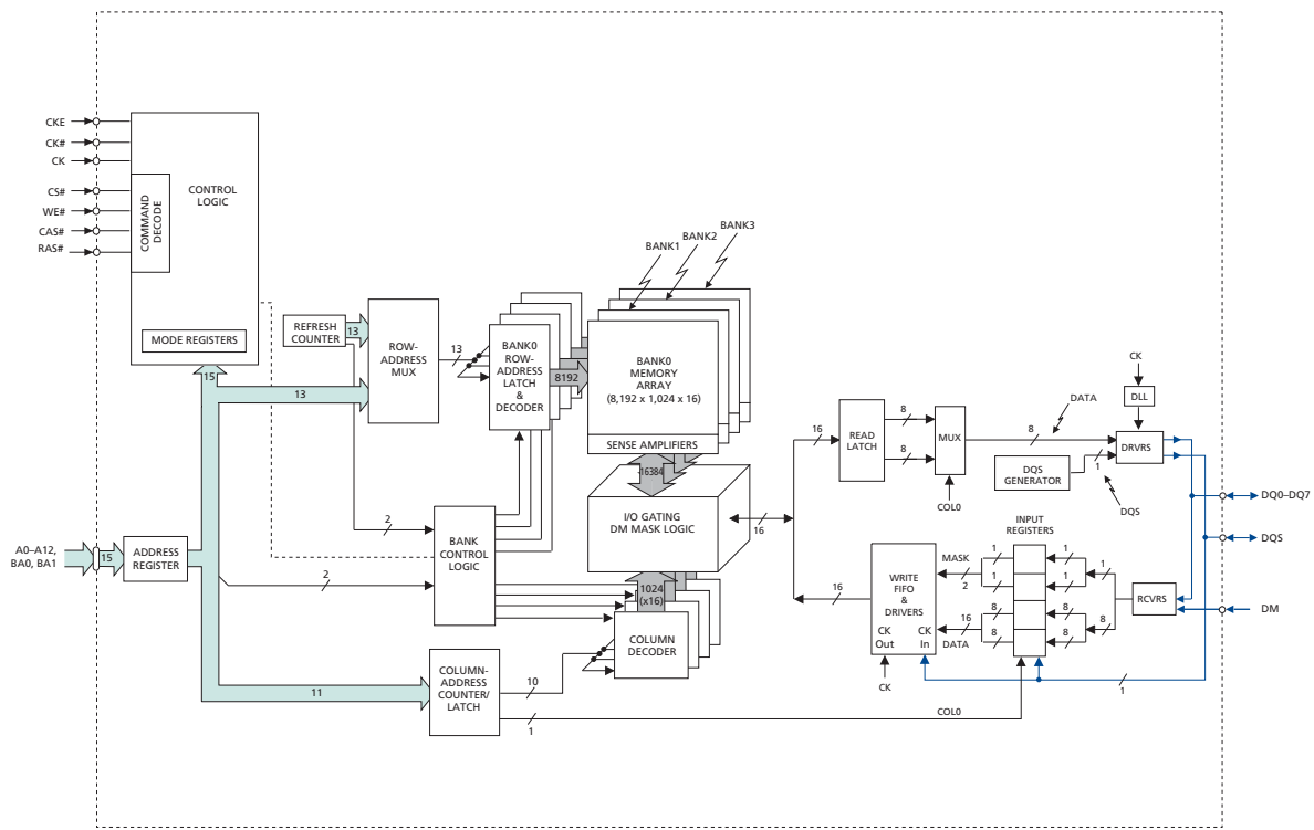
Figure 5: 32 Meg x 16 Functional Block Diagram
