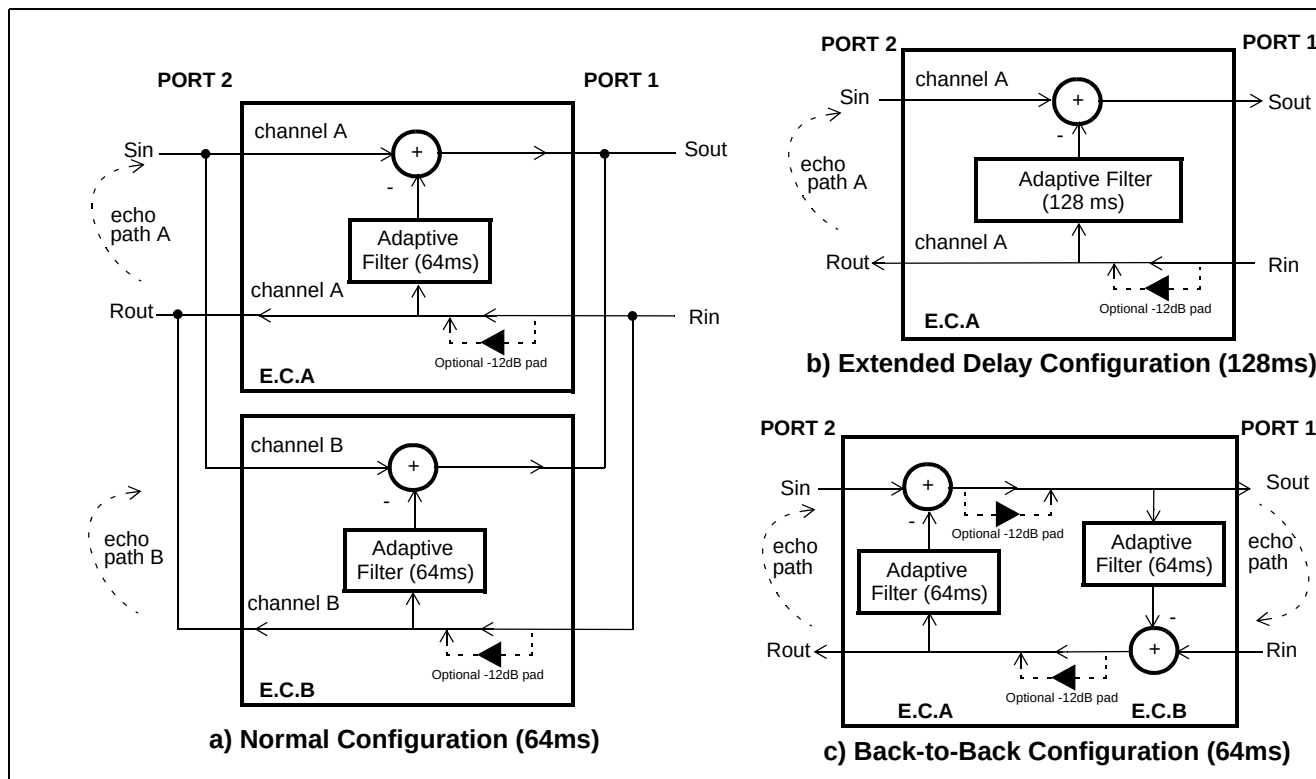
Figure 3 - Device Configuration
