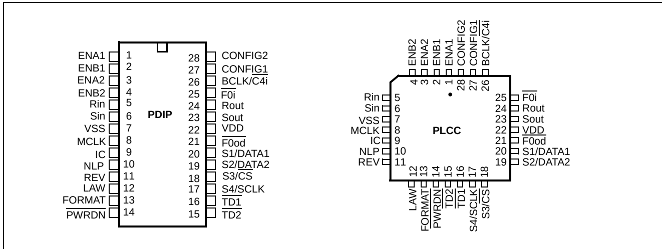
Figure 2 - Pin Connections
