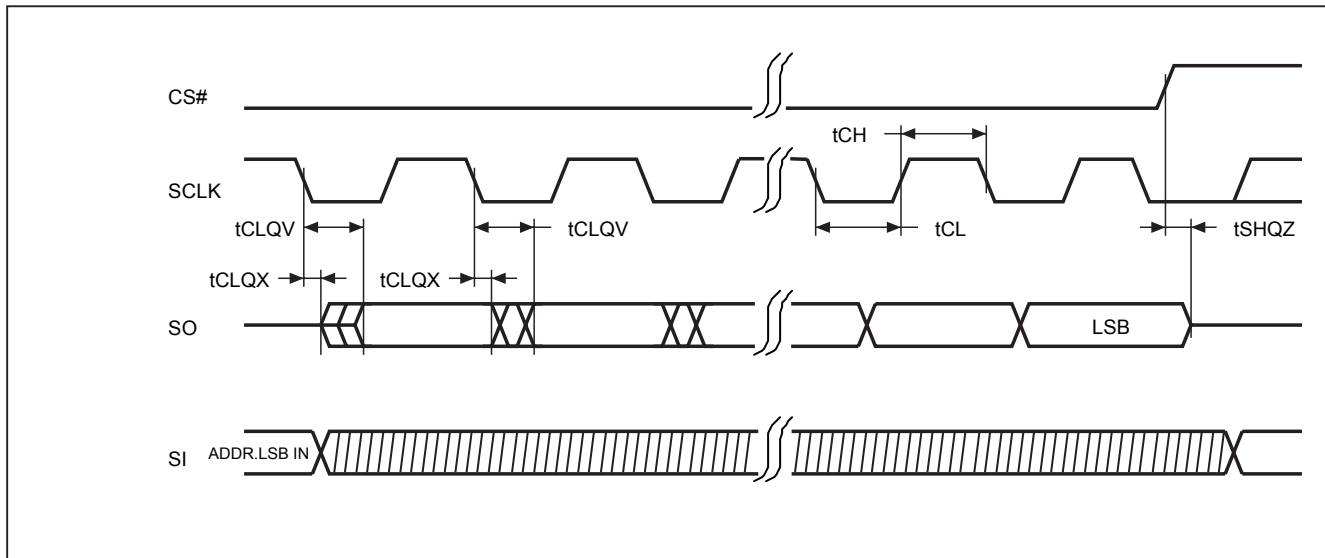
Figure 49. Output Timing
