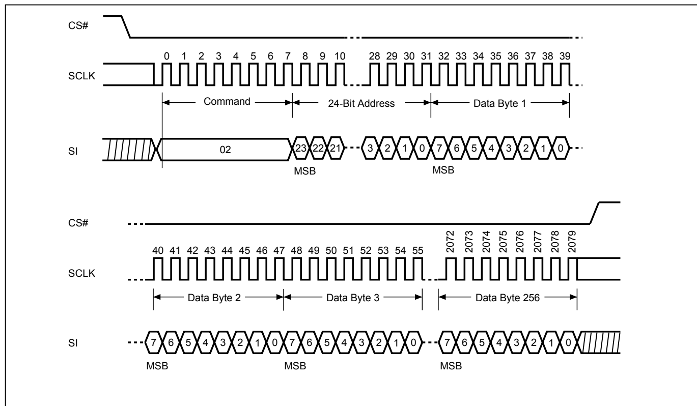
Figure 23. Page Program (PP) Sequence (Command 02)
