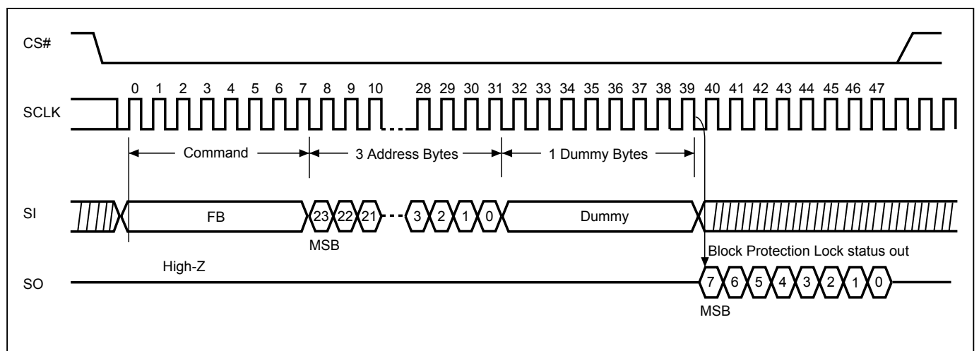
Figure 16. Read Block Protection Lock Status (RDBLOCK) Sequence (Command FB)
