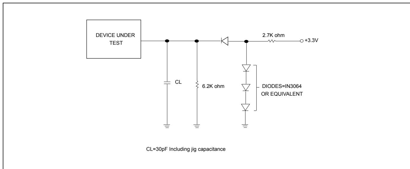
Figure 5. OUTPUT LOADING
