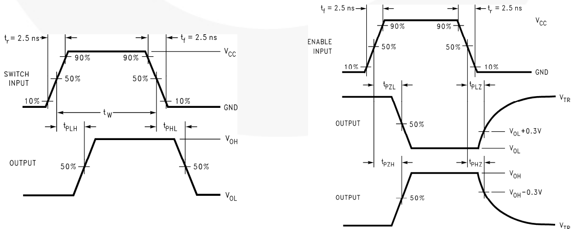
Figure 5. AC Waveforms
