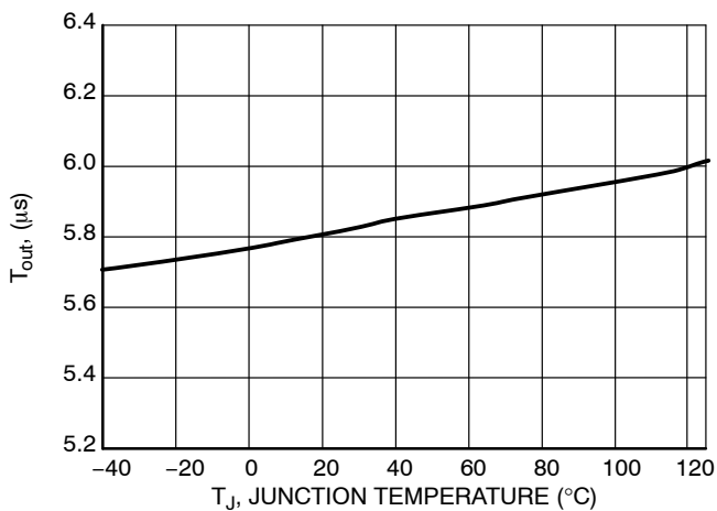
Figure 19. T_{out} vs. Junction Temperature
