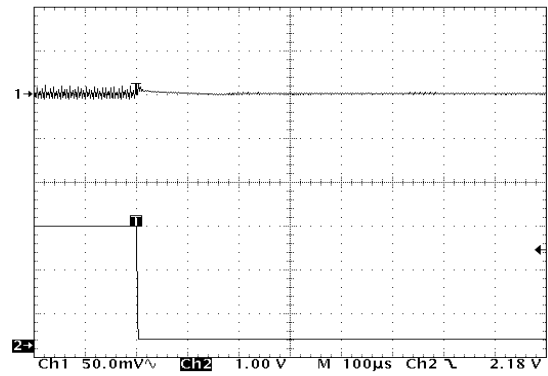
V_{IN} = 1.5\text{ V} , L = 22\text{ }\mu\text{H} 1. V_{OUT} = 3.0\text{ V} (AC coupled), 50 mV/div 2. I_O = 30\text{ mA} to 3.0\text{ mA}
