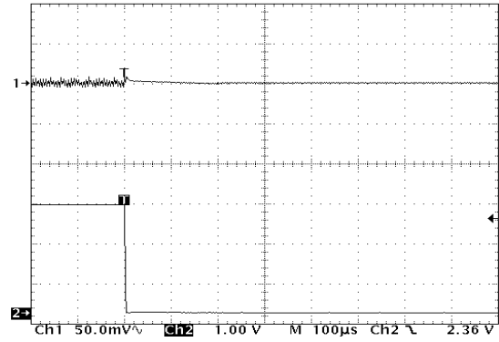
V_{IN} = 1.2\text{ V} , L = 22\text{ }\mu\text{H} 1. V_{OUT} = 1.9\text{ V} (AC coupled), 50 mV/div 2. I_O = 30\text{ mA} to 3.0\text{ mA}
