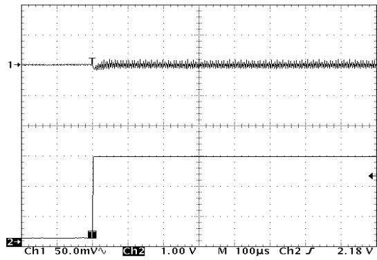
V_{IN} = 1.5\text{ V} , L = 22\text{ }\mu\text{H} 1. V_{OUT} = 3.0\text{ V} (AC coupled), 50 mV/div 2. I_O = 3.0\text{ mA} to 30\text{ mA}
