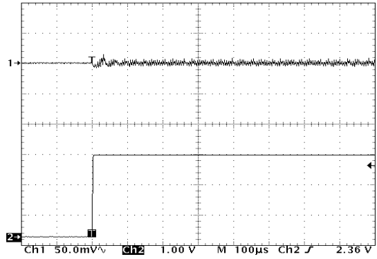
V_{IN} = 1.2\text{ V} , L = 22\text{ }\mu\text{H} 1. V_{OUT} = 1.9\text{ V} (AC coupled), 50 mV/div 2. I_O = 3.0\text{ mA} to 30\text{ mA}
