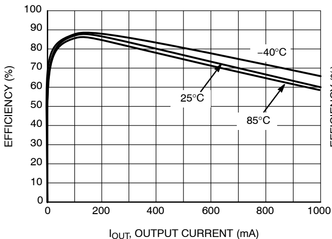
Figure 11. Efficiency vs. Output Current ( V_{IN} = 3.3\text{ V} , V_{OUT} = 1.2\text{ V} )
