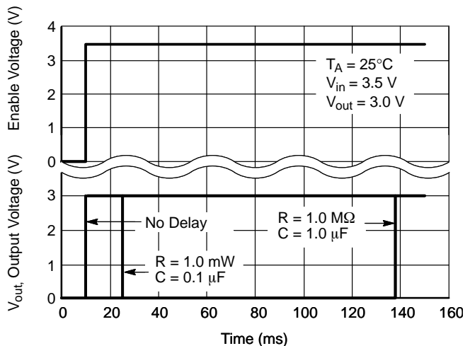
Figure 21. Delayed Turn-on
