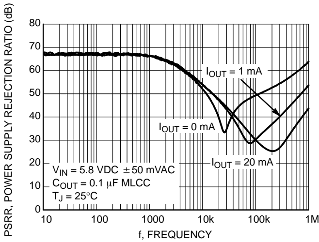
Figure 12. Power Supply Rejection Ratio C_{out} = 0.1\text{ }\mu\text{F}
