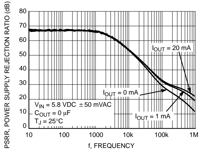
Figure 11. Power Supply Rejection Ratio C_{out} = 0\text{ }\mu\text{F}
