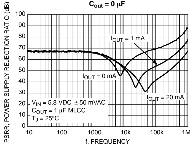
Figure 13. Power Supply Rejection Ratio C_{out} = 1\text{ }\mu\text{F}
