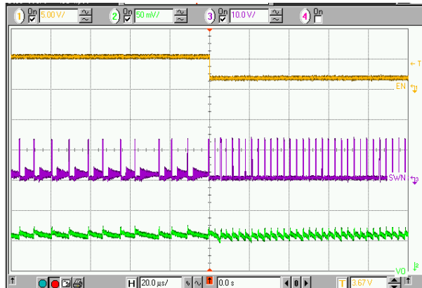
Top to Bottom: EN, SWM, V O Figure 12. On Line Mode Change (DCM → CCM)
