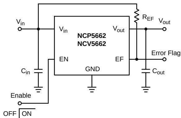
Figure 1. Typical Application Schematic, Fixed Output
