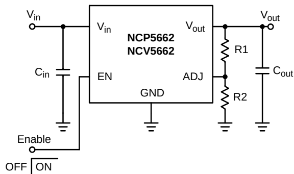
Figure 2. Typical Application Schematic, Adjustable Output
