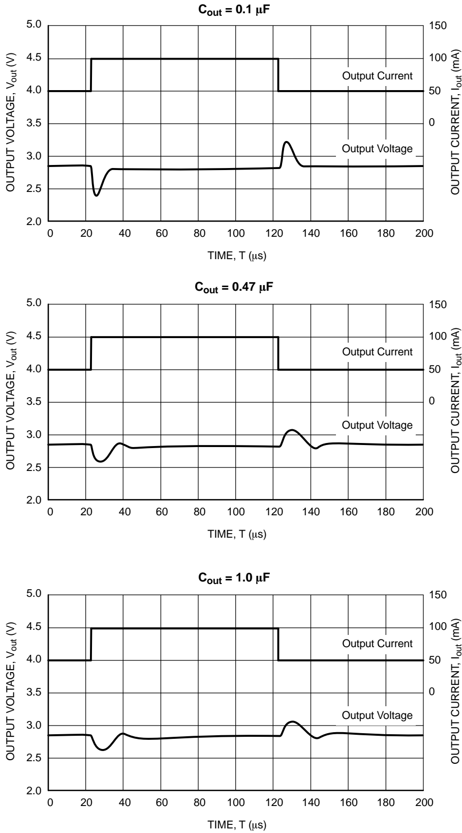
Figure 15. Load Transient Response ( V_{\text{out}} = 2.8 \text{ V} , t_r = t_f = 5.0 \mu\text{s} , V_{\text{in}} = 3.8 \text{ V} )
