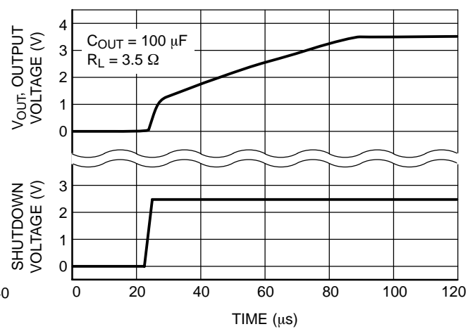
Figure 8. Start-up Transient
