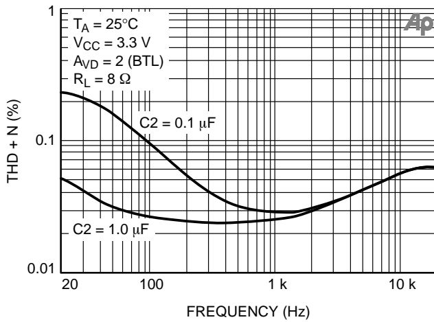
Figure 8. THD + N vs. Frequency ( P_L = 350 mW)
