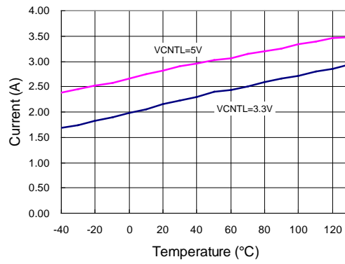
Sinking Current Limit vs. Temperature
