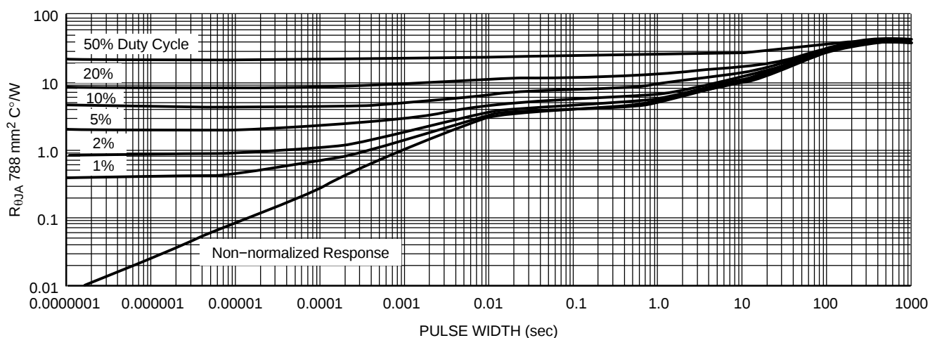
Figure 36. Duty Cycle for 1" Spreaders Boards, D²PAK 5-Lead
