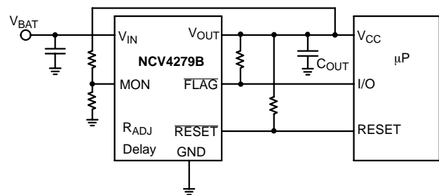
Figure 13. FLAG/Monitor Function
