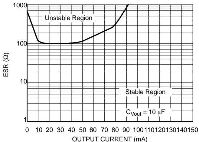
Figure 8. Output Capacitor ESR
