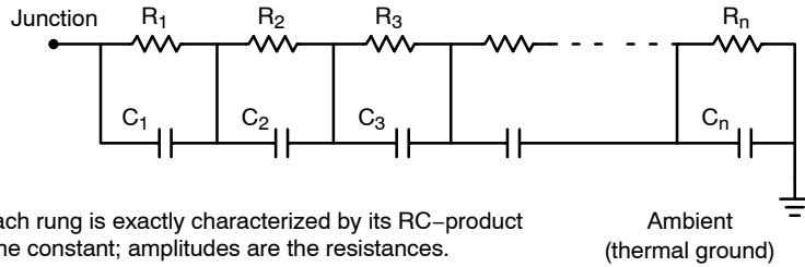
Figure 27. Non-Grounded Capacitor Thermal Ladder (“Foster” Ladder)
