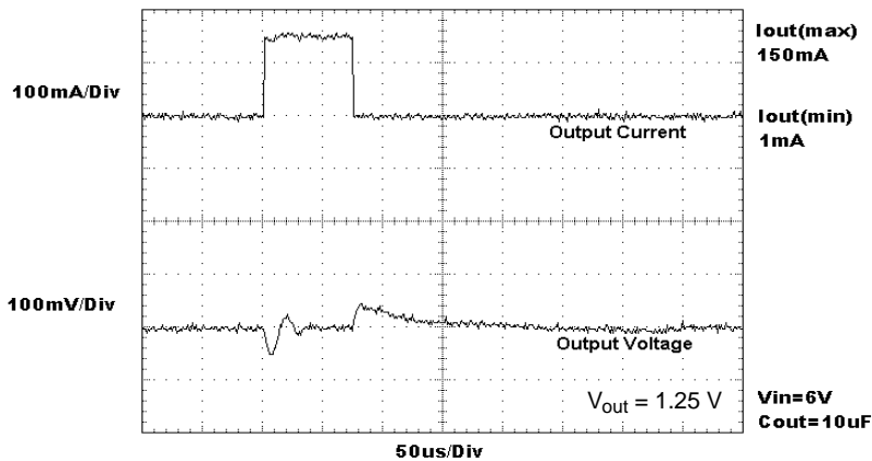
Figure 33. Load Transient Response ( 10\ \mu\text{F} )
