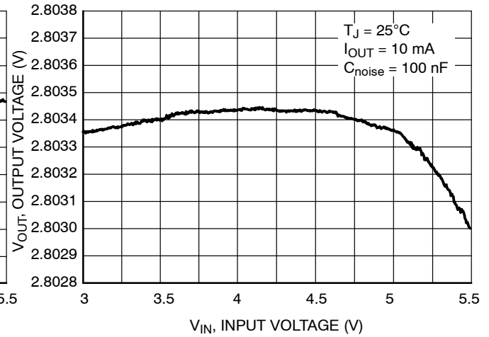
Figure 48. Output Voltage vs. Input Voltage, V_{OUT} = 2.8\text{ V} , C_{OUT} = 1\ \mu\text{F}
