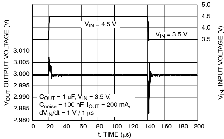
Figure 33. Line Transient Response, V_{\text{OUT}} = 3.0 \text{ V} , C_{\text{OUT}} = 1 \mu\text{F} , I_{\text{OUT}} = 200 \text{ mA}
