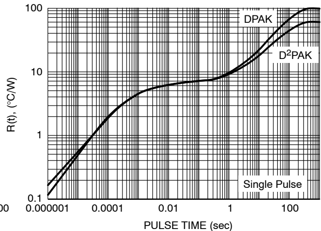
Figure 38. NCV8675 @ PCB Cu Area 100 mm 2 PCB Cu thk 1 oz
