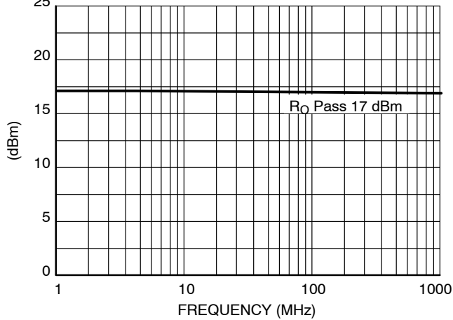
Figure 42. Typical R_O Pin Susceptibility
