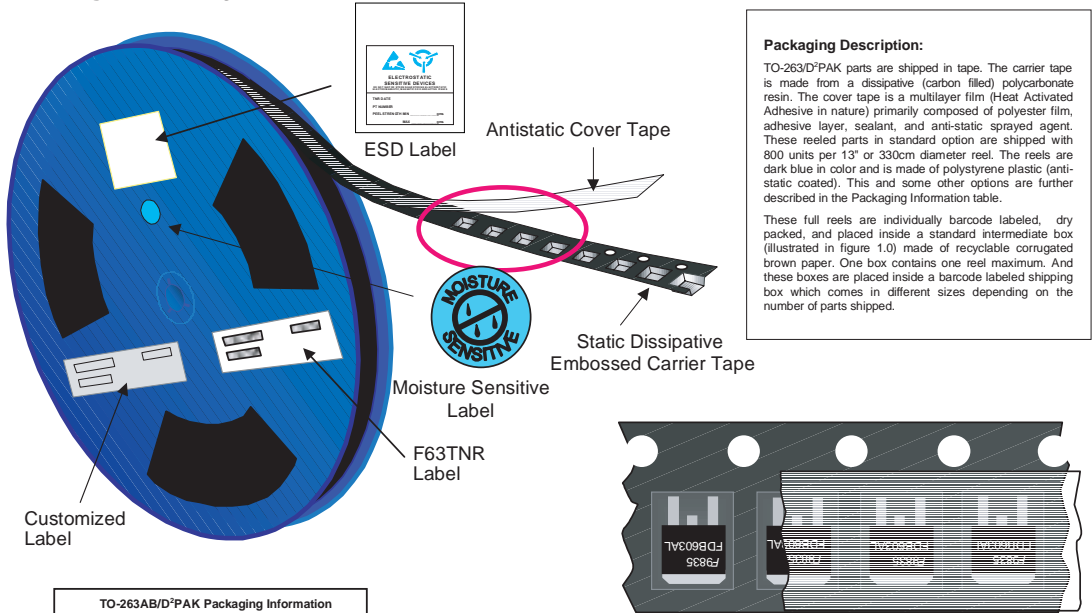
TO-263AB/D 2 PAK Unit Orientation
