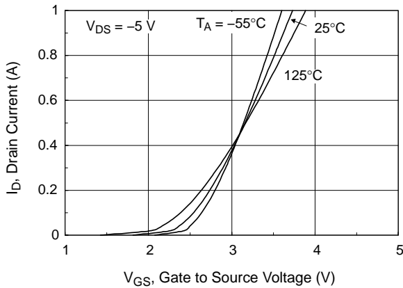
Figure 5. Transfer Characteristics
