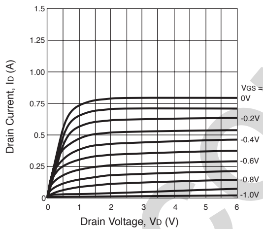
DRAIN CURRENT vs. DRAIN VOLTAGE
