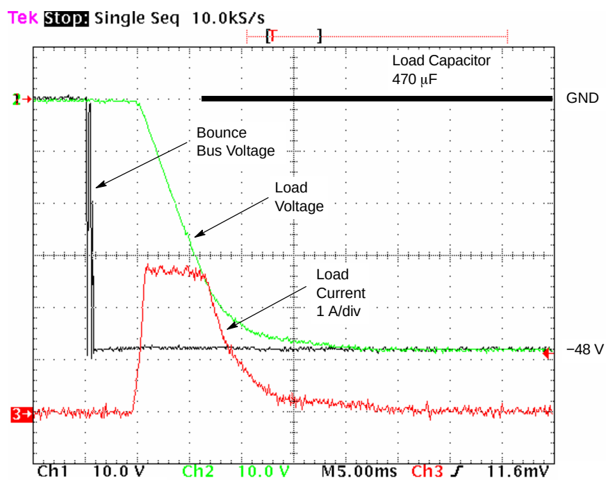
Figure 9. Turn On Waveforms for 470 \mu F Load Capacitor
