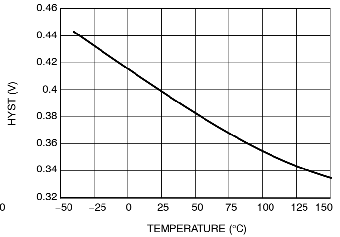
Figure 7. UVLO Hysteresis
