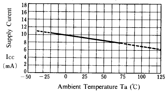
Supply Current vs. Temperature ( V^+/V^- = \pm 15V )
