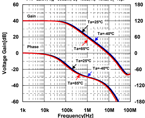
40dB Gain/Phase vs. Frequency (Temperature)
