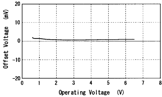
Offset Voltage vs. Operating Voltage VIN=0.1V
