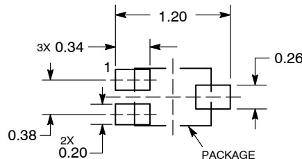
DIMENSIONS: MILLIMETERS
