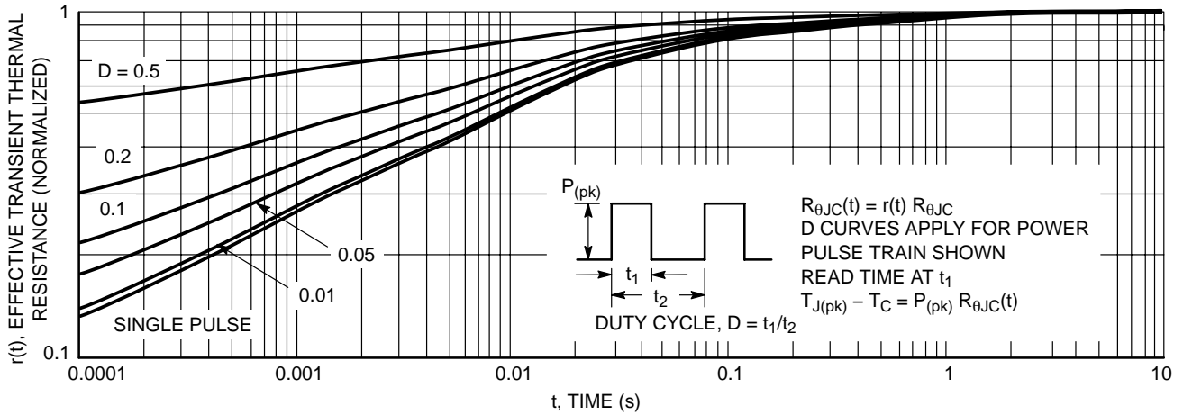
Figure 12. Thermal Response
