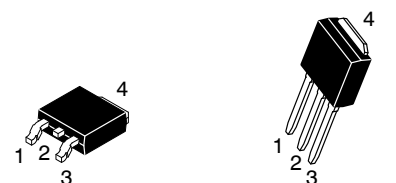
DPAK CASE 369C (Surface Mounted) STYLE 2
