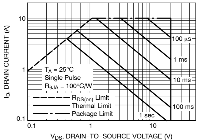
Figure 12. Safe Operating Area (SOA)
