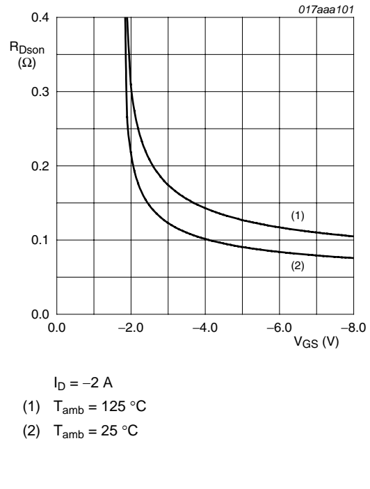
Fig 9. Drain-source on-state resistance as a function of gate-source voltage; typical values
