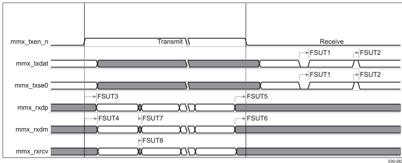
Figure 6-46. Low-/Full-Speed USB – Unidirectional TLL 6-pin Mode
