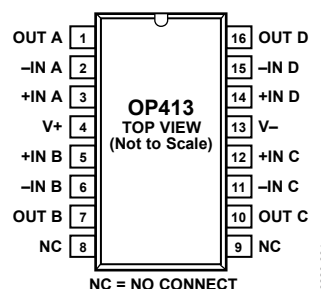
Figure 4. 16-Lead Wide-Body SOIC_W
