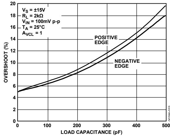
Figure 34. Small-Signal Overshoot vs. Load Capacitance @ \pm 15 V
