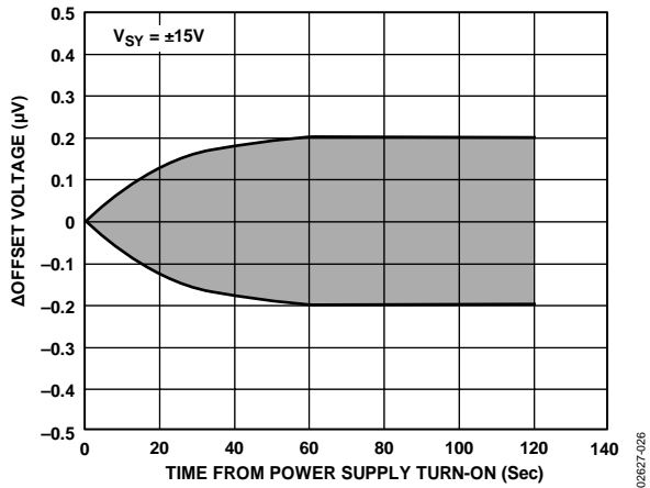
Figure 26. Warm-Up Drift
