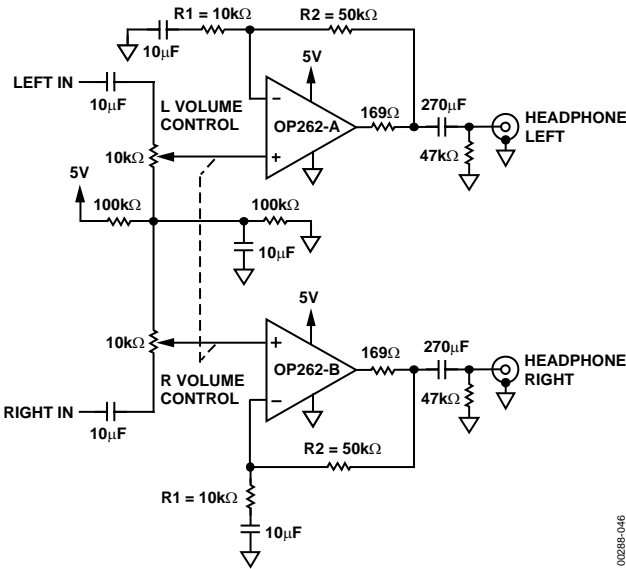
Figure 43. Headphone Output Amplifier
