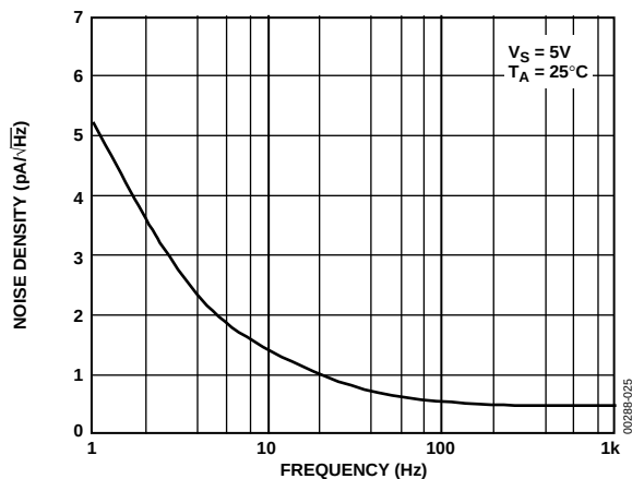
Figure 22. Current Noise Density vs. Frequency
