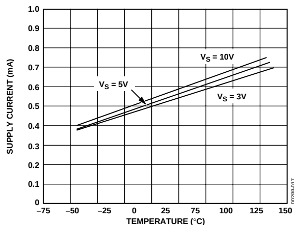
Figure 14. Supply Current/Amplifier vs. Temperature
