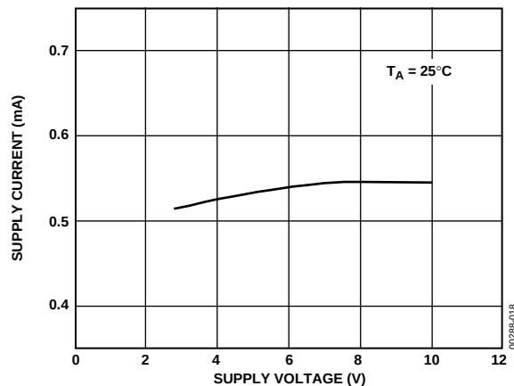
Figure 15. OP462 Supply Current/Amplifier vs. Supply Voltage
