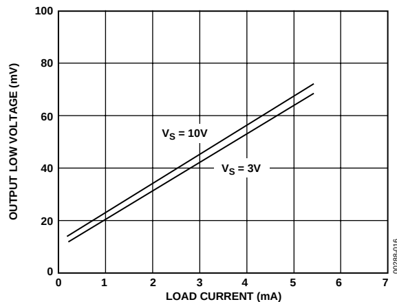
Figure 13. Output Low Voltage to Supply Rail vs. Load Current
