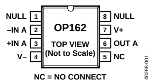
Figure 1. 8-Lead Narrow-Body SOIC (S Suffix)
