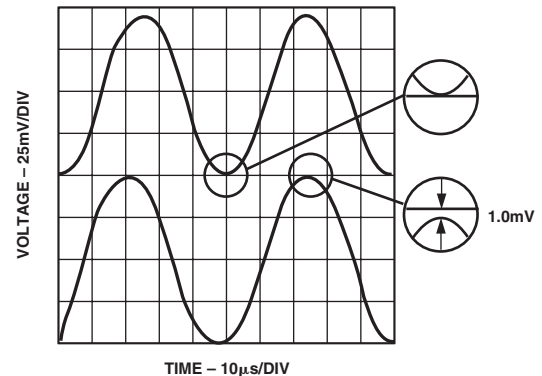
Figure 6. Rail-to-Rail Operation
