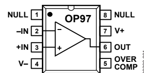
Figure 1. 8-Lead PDIP (P Suffix) 8-Lead SOIC (S Suffix)
