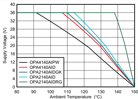
Figure 7-4. Maximum Supply Voltage vs Temperature, DC Worst-Case
