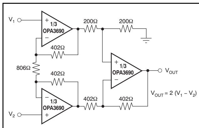
Figure 41. Instrumentation Amplifier
