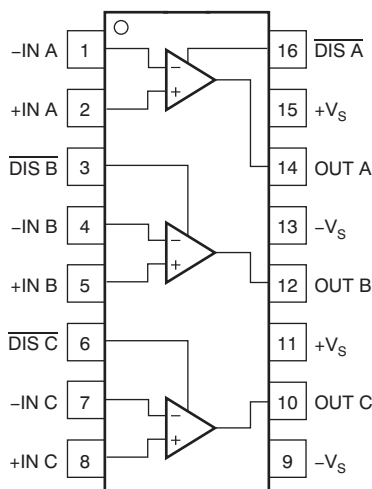
D AND DBQ PACKAGES SO-16 AND SSOP-16 (TOP VIEW)
