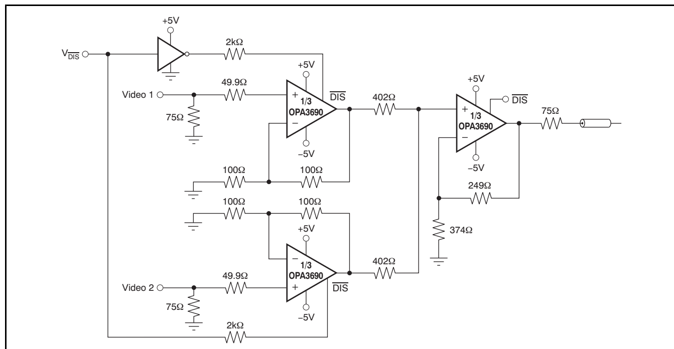
Figure 44. Buffered 2 x 1 Multiplexer
