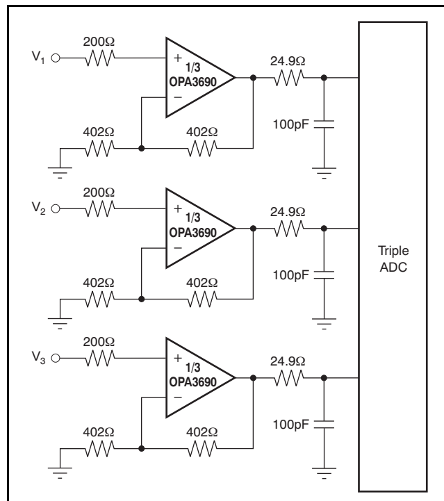
Figure 43. Triple ADC Driver
