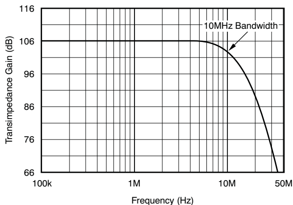
Frequency Response of 200-k \Omega Transimpedance Amplifier
