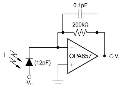
Wideband Photodiode Transimpedance Amplifier
