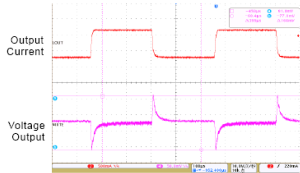
Load Transient I o =0-1A, V o =1.2V, V in =3.6V
