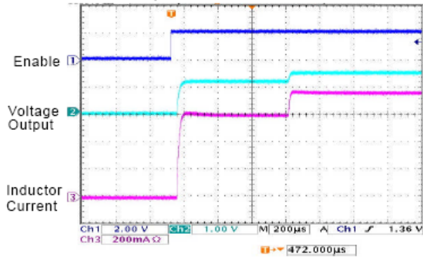
Start-up from Shutdown V o =1.8V, V in =3.6V
