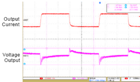
Load Transient I o =0-500mA, V o =3.3V, V in =5V
