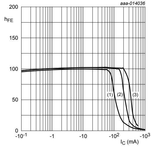
h_{FE} = f(I_C) T_{amb} = 25^\circ C (1) V_{CE} = -10\text{ V} (2) V_{CE} = -25\text{ V} (3) V_{CE} = -50\text{ V}
